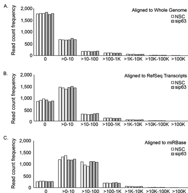
Figure 3. Alignment and quantitation to miRBase provides the most robust read quantitation. The frequency of raw read counts from each of the 3 biological replicates for the NSC and sip63 datasets is shown for (A) Whole Genome, (B) RefSeq and (C) miRBase alignments after quantitation using the miRBase reference. Open and gray bars indicate NSC and sip63 samples, respectively.
